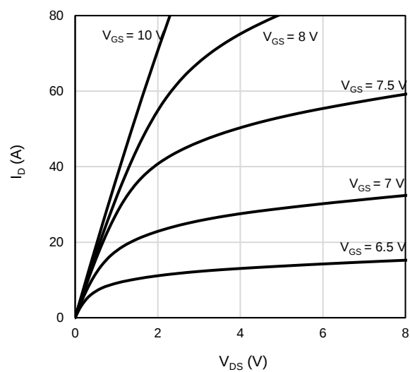
Figure 1: On-Region Characteristics
